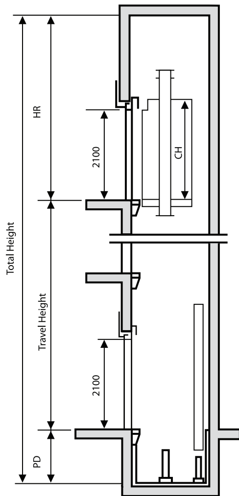
HOISTWAY SECTION (mm.)
