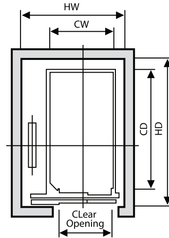
SHAFT DIMENSION
