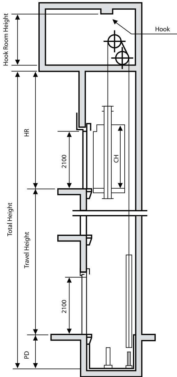
HOISTWAY SECTION (mm.)
